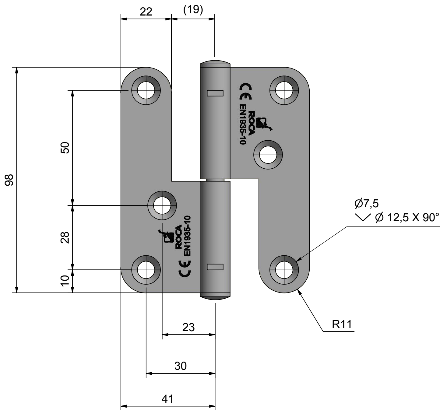
931315 Right handed
