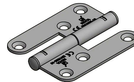
931316 Left handed
